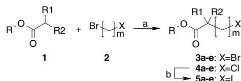
Scheme 2. Reagents and condition: (a) LDA, THF, -60^\circ\text{C} to rt; (b) NaI, 2-butanone, \Delta .
