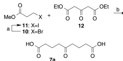
Scheme 5. Reagents and conditions: (a) \text{NaI} , acetone, rt, 95%; (b) (1) \text{NaOEt} , 90^\circ\text{C} , (2) \text{HCl} (concd), \text{H}_2\text{O} , \Delta , 44%.
