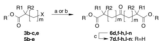
Scheme 3. Symmetrical ketones. Reagents and conditions: (a) 6d,g,h,m,n : Method A: 11 (1) NaH, TosMIC, Bu 4 NI, DMSO, rt, (2) HCl (concd), CH 2 Cl 2 , rt; (b) 6f,i : Method B: 11 (1) KO t Bu, TosMIC, DMAc, 0^\circ\text{C} –rt, (2) HCl (concd), CH 2 Cl 2 , rt; (c) 6d,i : Method E: 11 HCO 2 H, rt, 6f,g,m,n : Method D: 11 LiOH, EtOH/H 2 O, \Delta , 6h : KOH, EtOH/H 2 O, rt.
