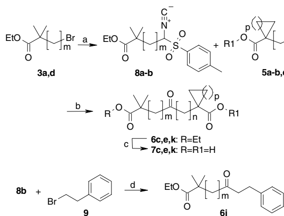
Scheme 4. Asymmetrical ketones. Reagents and conditions: (a) \text{K}_2\text{CO}_3 , \text{Bu}_4\text{NI} , DMF, rt, 8a ( m = 4 ) 67%, 8b ( m = 5 ) 61%; (b) Method C: 11 (1) \text{KOtBu} , TosMIC, DMAc, 0^\circ\text{C} –rt, (2) \text{HCl} (concd), \text{CH}_2\text{Cl}_2 , rt; (c) 6c,k : Method F: 11 (1) \text{HCO}_2\text{H} , rt, (2) \text{NaOH} , \text{EtOH}/\text{H}_2\text{O} , \Delta , 6c : Method D: 11 \text{LiOH} , \text{EtOH}/\text{H}_2\text{O} , \Delta ; (d) Method A: 11 (1) \text{NaH} , TosMIC, \text{Bu}_4\text{NI} , DMSO, rt, (2) \text{HCl} (concd), \text{CH}_2\text{Cl}_2 , rt, 68%.
