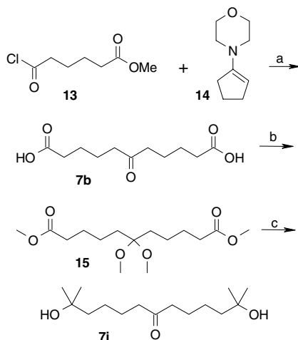
Scheme 6. Reagents and conditions: (a) (1) Et 3 N, Δ, (2) 1 M HCl, Δ, (3) 17 M KOH, 100 °C, 69%; (b) CH(OMe) 3 , TsOH, MeOH, Δ, 85%; (c) (1) MeMgCl, Et 2 O/THF, 0 °C–rt, (2) 1 M HCl, rt, 93%.
